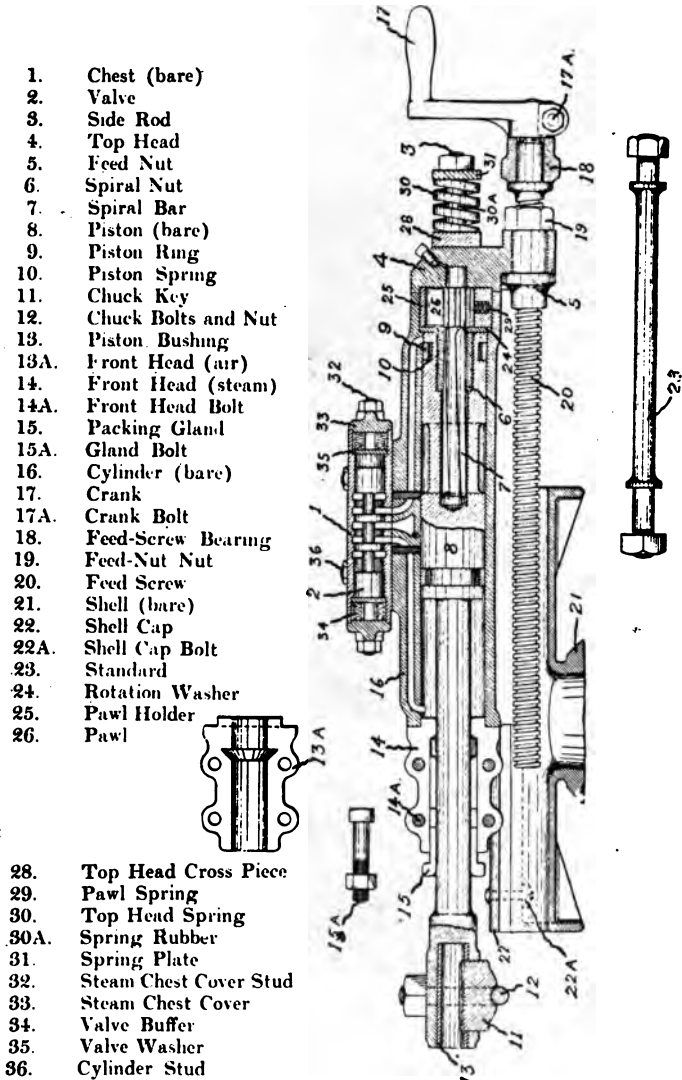
Fig. 17. Wood-Rock Drill.
